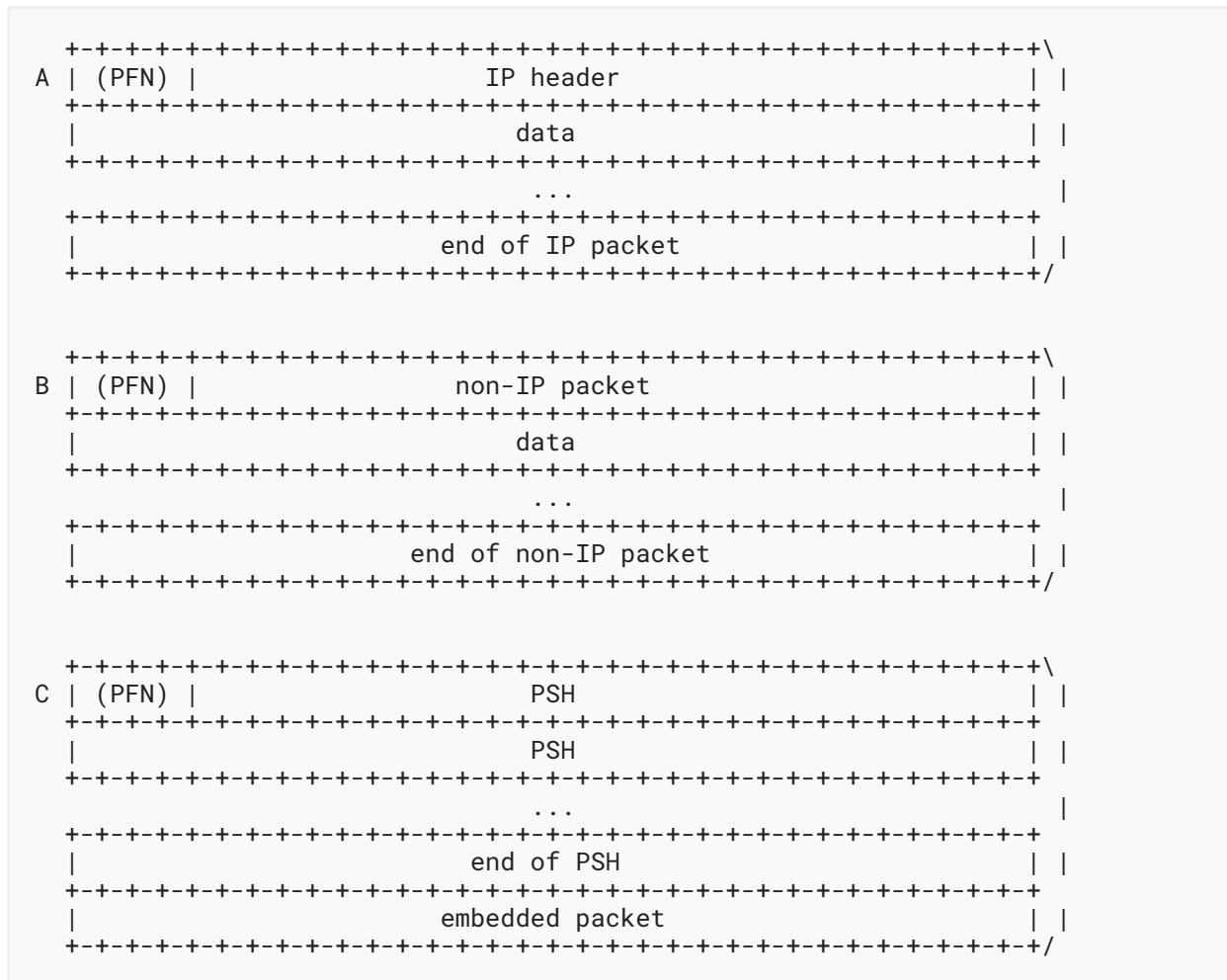
Figure 2: Examples of an MPLS Packet Payload With and Without Post-Stack Header
